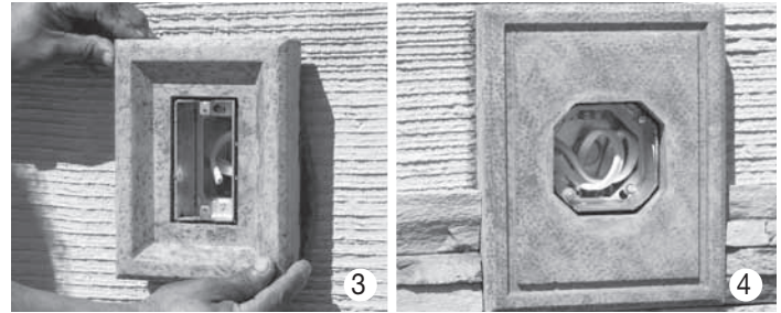
Center Electrical Box Stone over the extension box. Level and plumb. Use removable shims if required.
