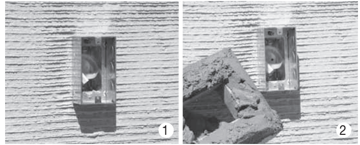
Attach UL-listed extension box to pre-wired and mounted electrical box.
